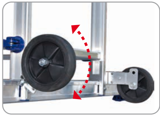
Quick castors lifting system. The ladders don't slip when they're in the positions: double section ladder and simple one (Patent).
