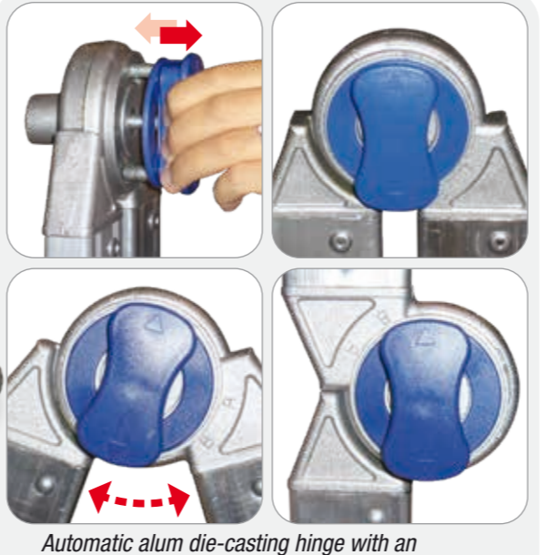
Automatic alum die-casting hinge with an inner steel plate strengthening.
