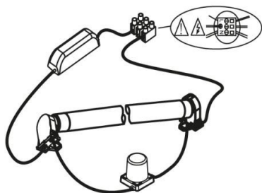
Before retrofit – existing fitting
